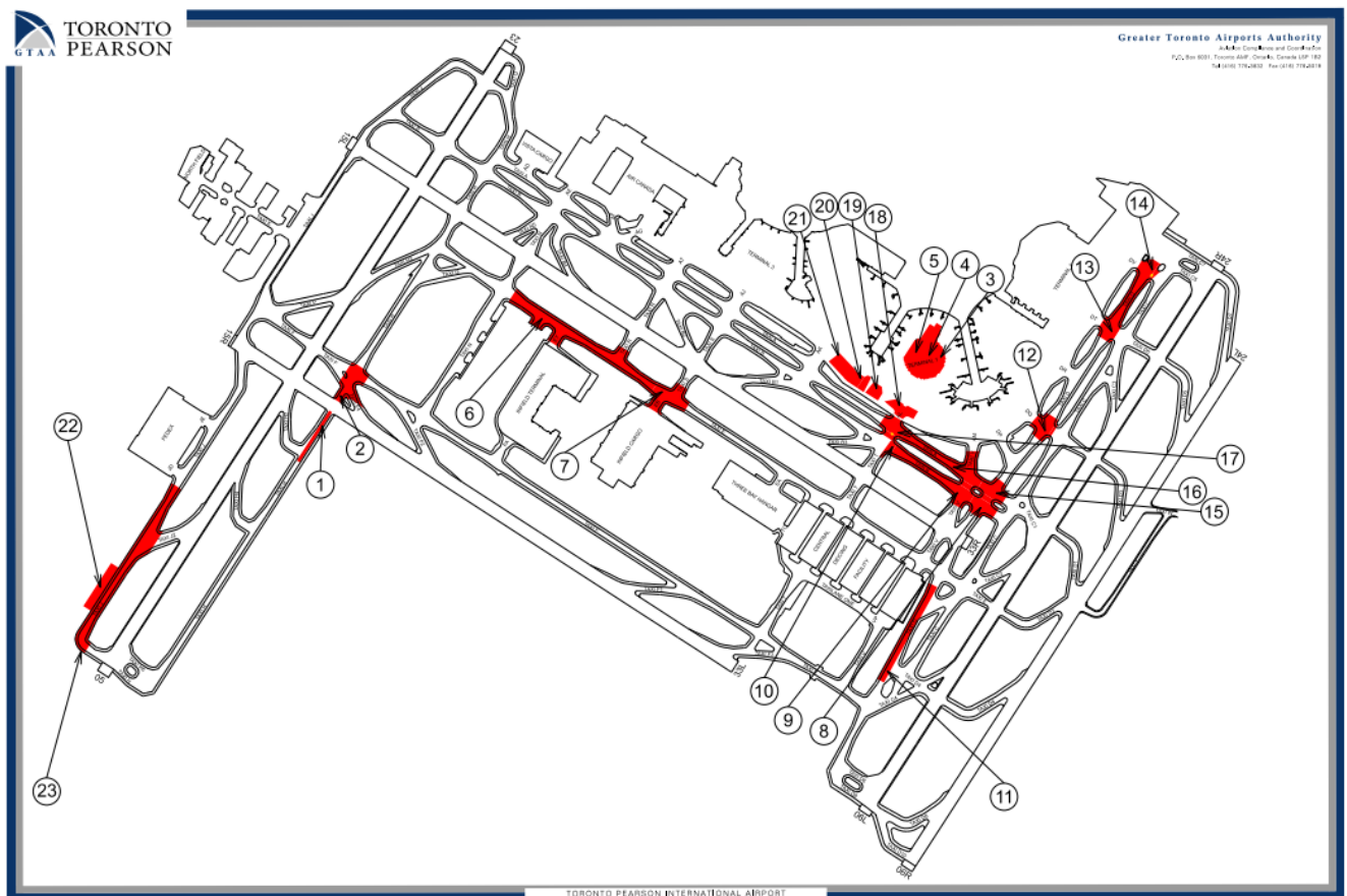
Figure 1: CYYZ Runway and Taxiway Identification Diagram
