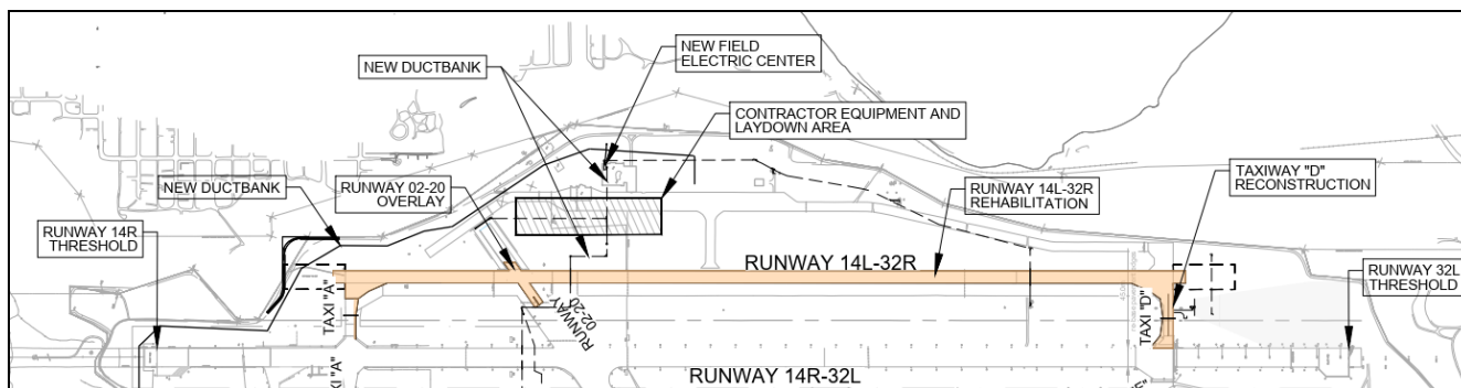
Figure 1: Taxiway D in the Extension of Runway 14L/32R
