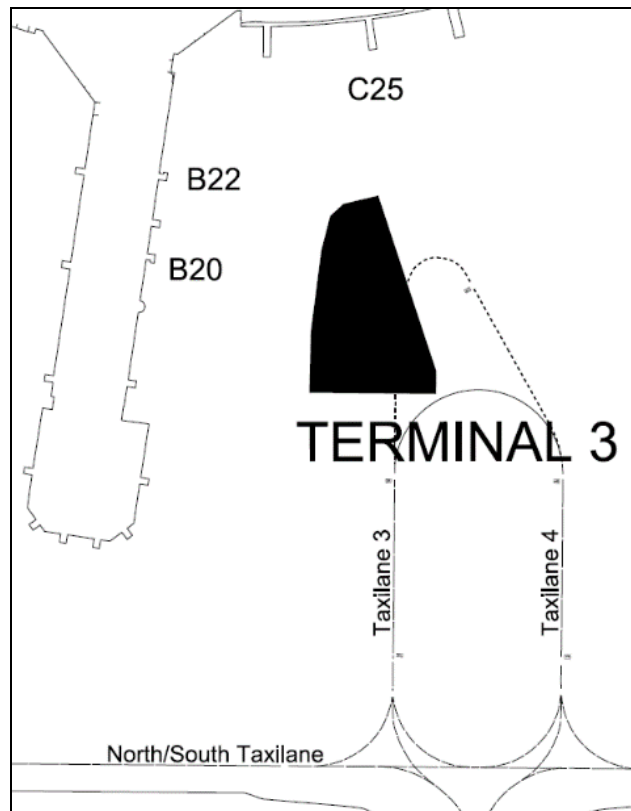
Figure 8: Taxilane 3 Construction Area
