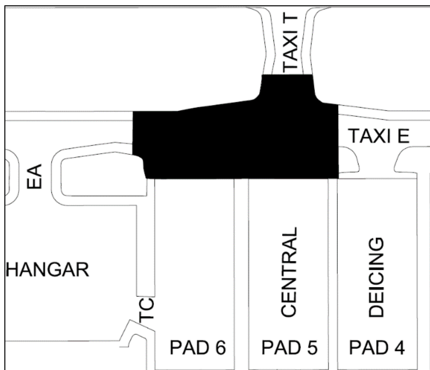
Figure 17: Taxiway E Construction Area
