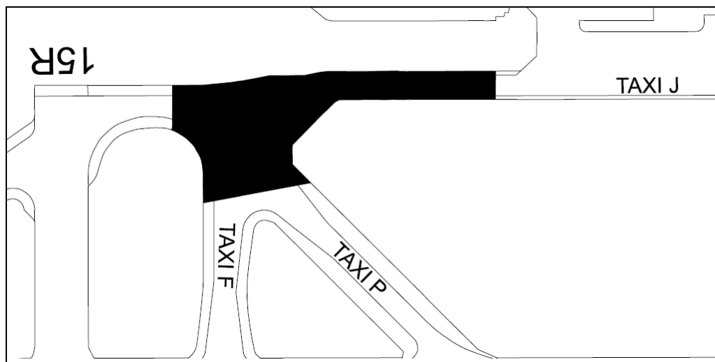
Figure 11: Taxiway J Construction Area
