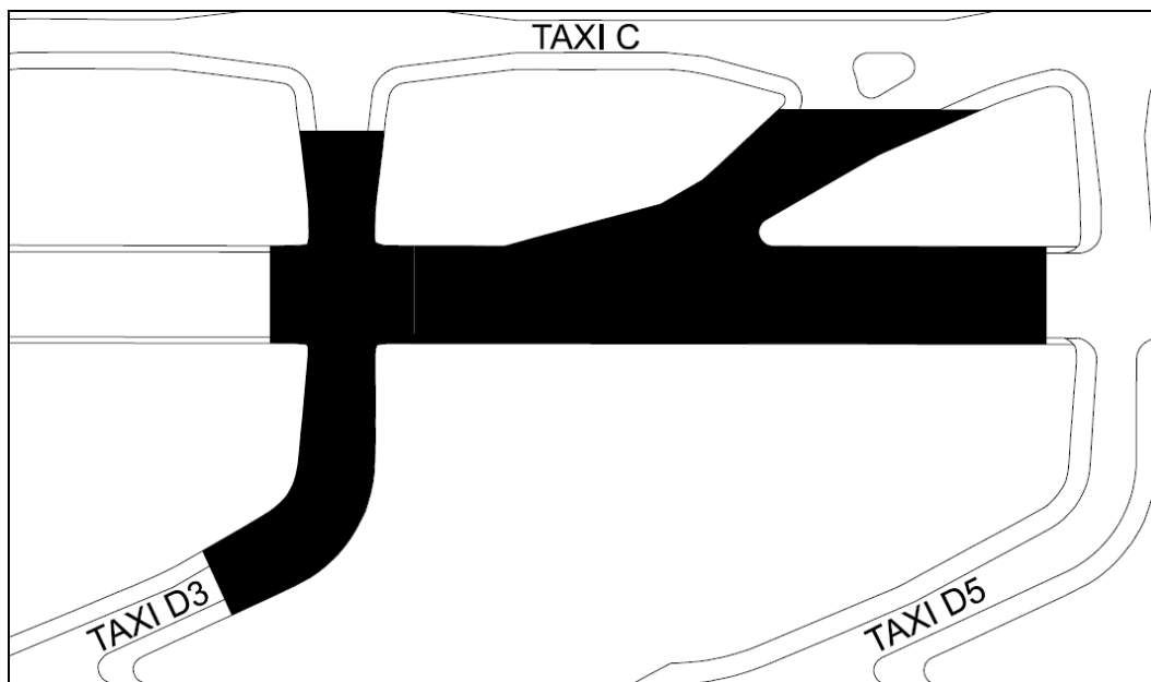
Figure 5: Runway 06L/24R Construction Area
