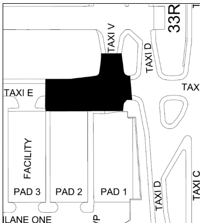
Figure 15: Taxiway E Construction Area
