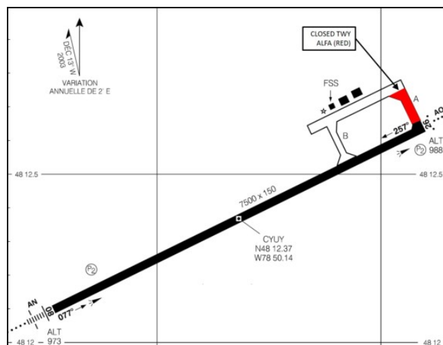
Figure 3: Construction Work for Phase 7.
