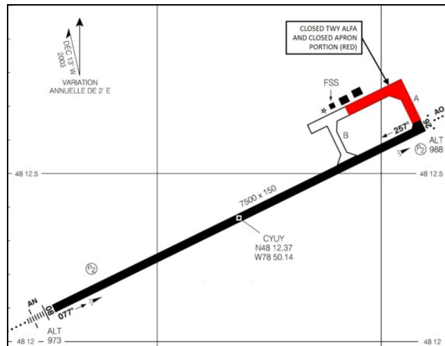
Figure 2: Construction Work for Phase 6.
