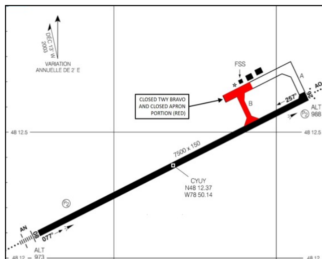
Figure 1: Construction Work for Phase 4 and Phase 5.
