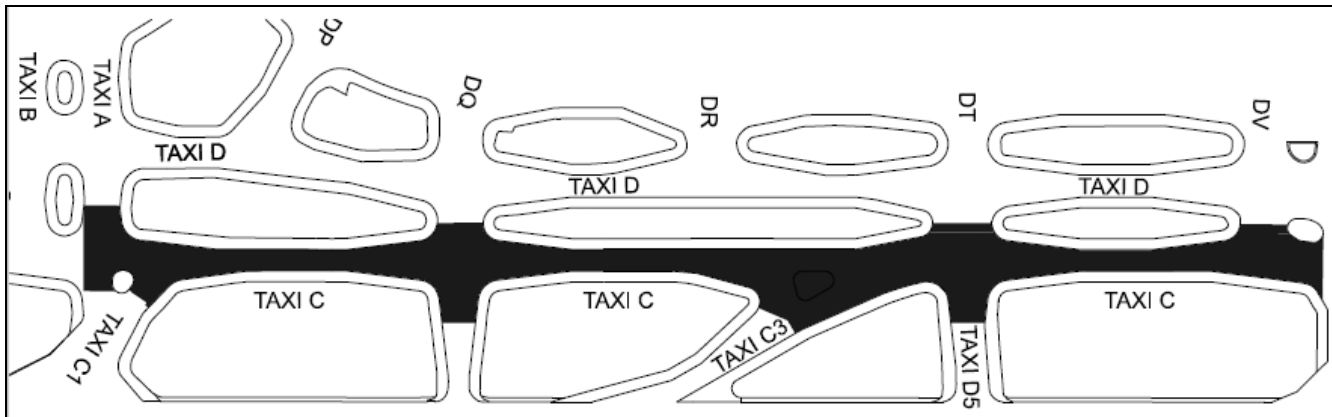
Figure 9: Taxiway CHARLIE Phase 5 Construction (Area 2)
