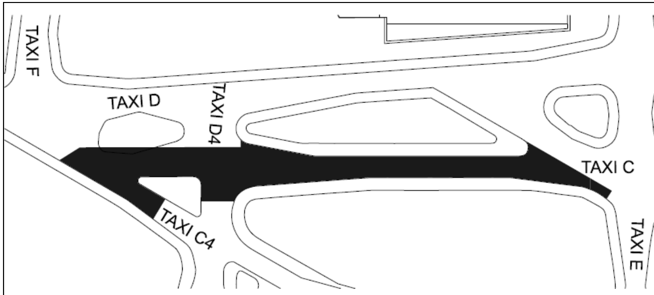
Figure 7: Taxiway CHARLIE Phase 3 Construction (Area 2)
