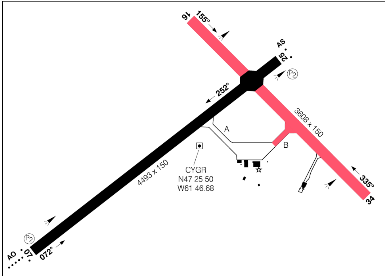
Figure 1. Overview of Phase 1A Construction Work
