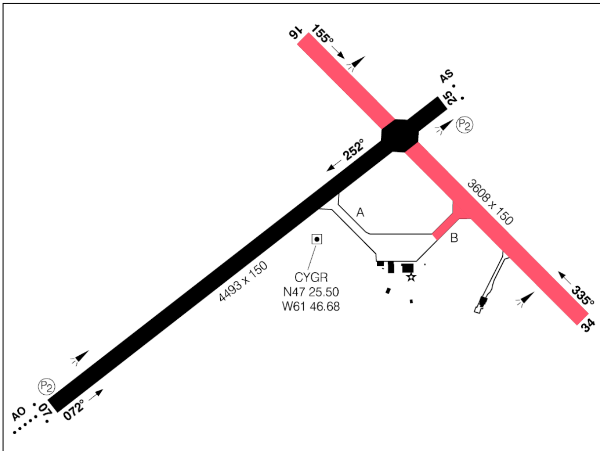
Figure 3. Overview of Phase 1B Construction Work
