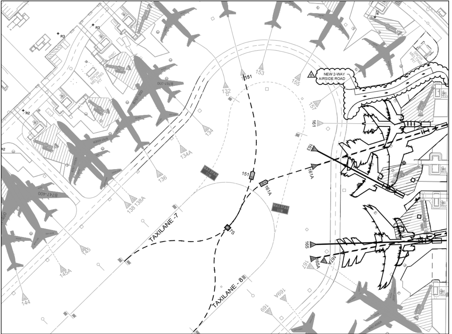
Figure 1: Transition Line 7S for Gate 151 and Gate 161A from Taxilane 7 and Taxilane 8.
