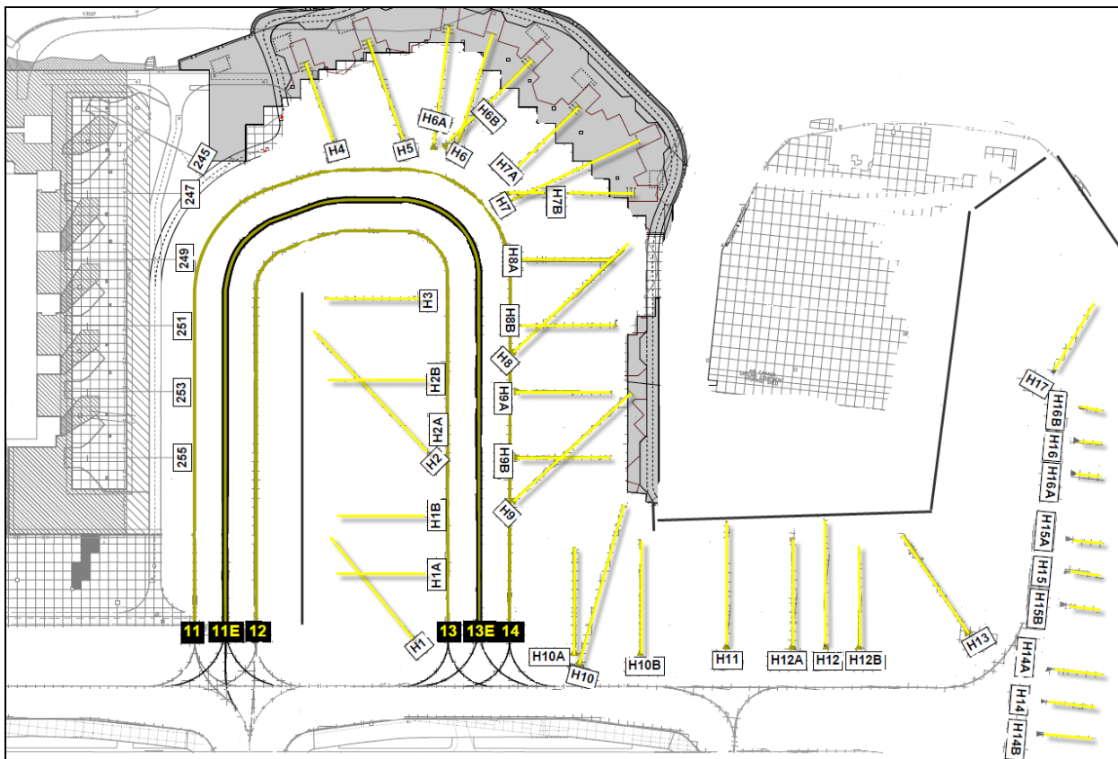
Figure 1: Terminal 1 East Apron Expansion Renamed Taxilanes
